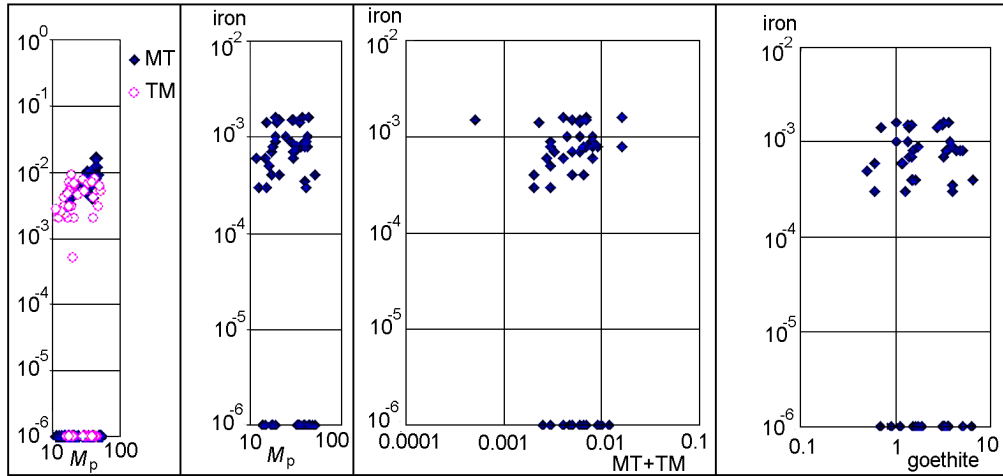
Figure 7. Correlation between paramagnetic magnetization ( M_p ), concentration of ferromagnetic Fe-hydroxides (goethite), magnetite, titanomagnetite, and metallic iron in sediments from the Gams section [Pechersky et al., 2006a, 2006b; Pechersky, 2008]; (D. M. Pechersky et al., in press, 2008b).
