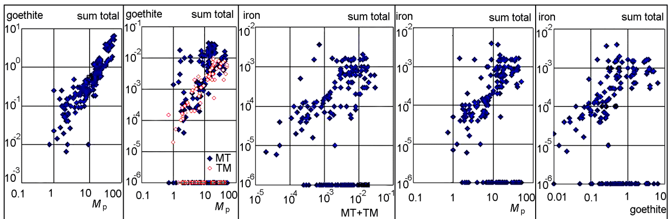
Figure 5. Correlation between paramagnetic magnetization ( M_p ) and concentration of ferromagnetic Fe-hydroxides (goethite), magnetite, titanomagnetite, and metallic iron in sediments. The data for the Gams, Koshak, Klyuchi, Teplovka, Tetrtskaro, and Khalats sections are combined [Molostovsky et al., 2006; Pechersky et al., 2006a, 2006b; Pechersky, 2008]; (D. M. Pechersky et al., in press, 2008a,b).
