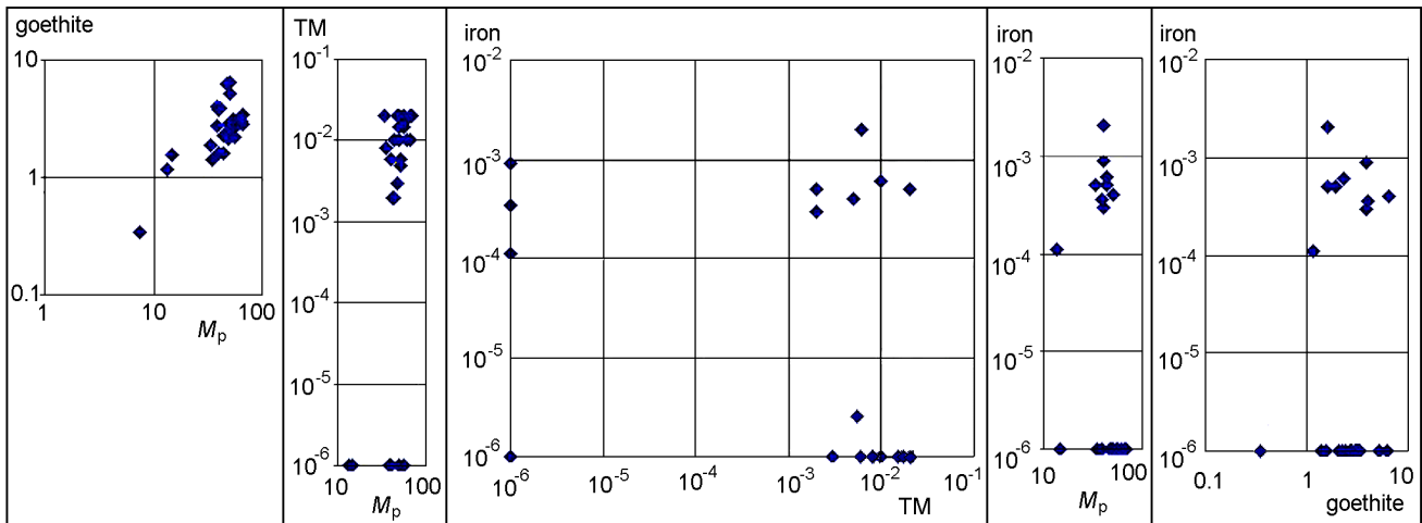
Figure 2. The relationship between concentrations of goethite, titanomagnetite and metallic iron in the boundary layer of the Gams section.
