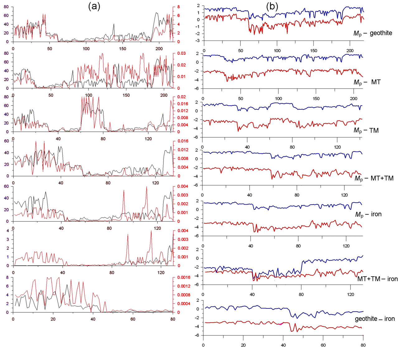
Figure 6. The paired rows of measured values from Figure 5: a, observed values; b, the logarithms.
