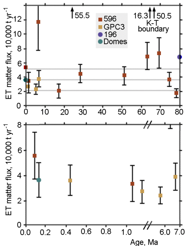
Figure 3. Cosmic dust accumulation rate in the Pacific columns of sediments [Peucker-Ehrenbrink, 1996].
