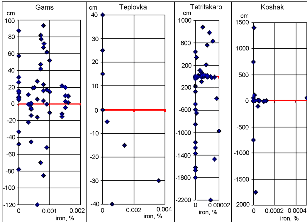
Figure 4. Examples of distribution of metallic iron in sediments close to the K-T boundary (red line).
