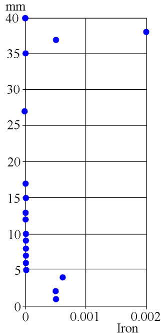
Figure 1. Distribution of metallic iron in the boundary layer as defined from three block samples from the Gams section (D. M. Pechersky et al., in press, 2008b).
