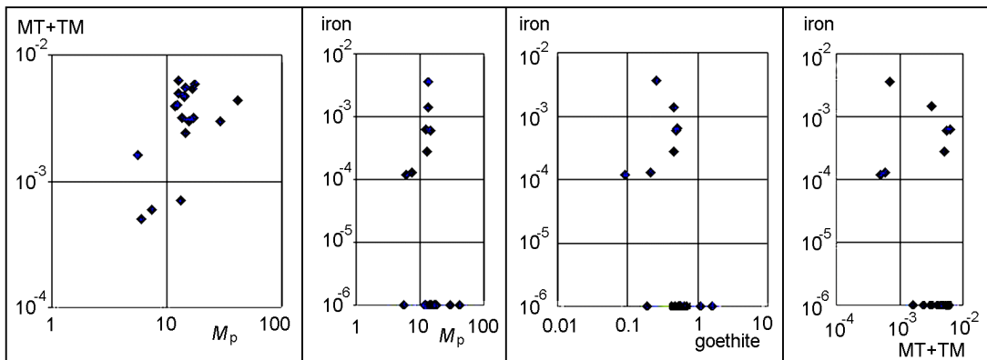
Figure 8. Correlation between paramagnetic magnetization ( M_p ), concentration of ferromagnetic Fe-hydroxides (goethite), magnetite, titanomagnetite, and metallic iron in sediments from the Klyuchi and Teplovka sections [Molostovsky et al., 2006; Pechersky, 2008].
