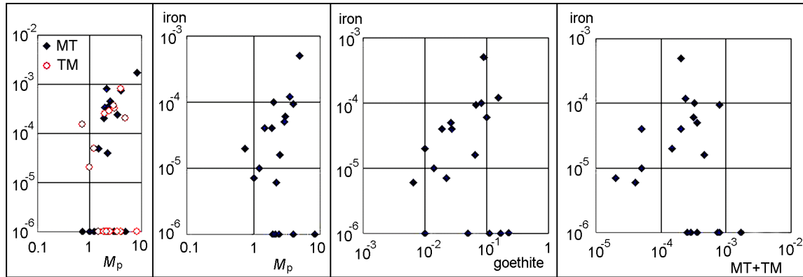
Figure 9. Correlation between paramagnetic magnetization ( M_p ), concentration of ferromagnetic Fe-hydroxides (goethite), magnetite, titanomagnetite, and metallic iron in sediments from the Koshak section [Pechersky et al. , 2006a, 2006b; Pechersky, 2008].
