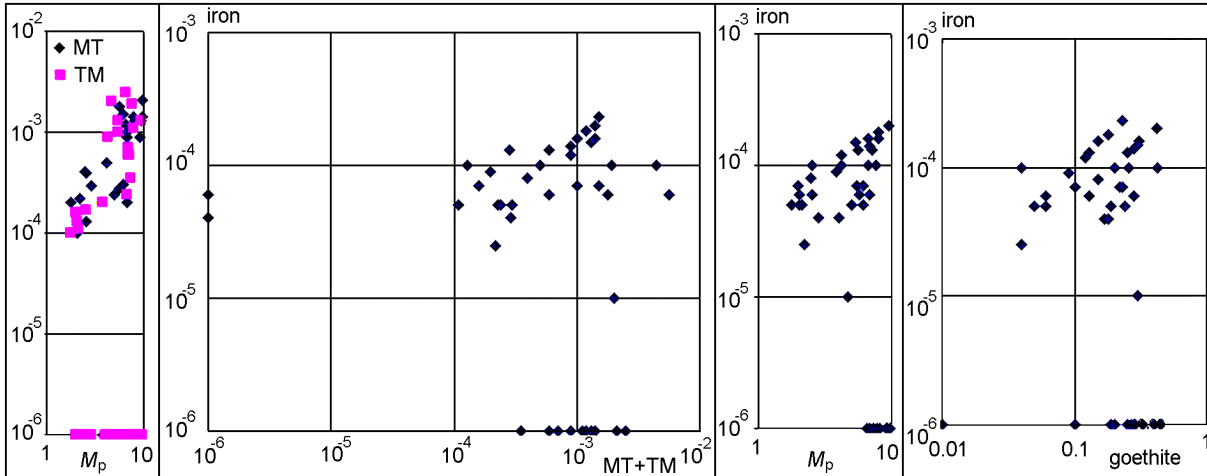
Figure 10. Correlation between paramagnetic magnetization ( M_p ), concentration of ferromagnetic Fe-hydroxides (goethite), magnetite, titanomagnetite, and metallic iron in sediments from the Tetrtskaro section (D. M. Pechersky et al., in press, 2008a).
