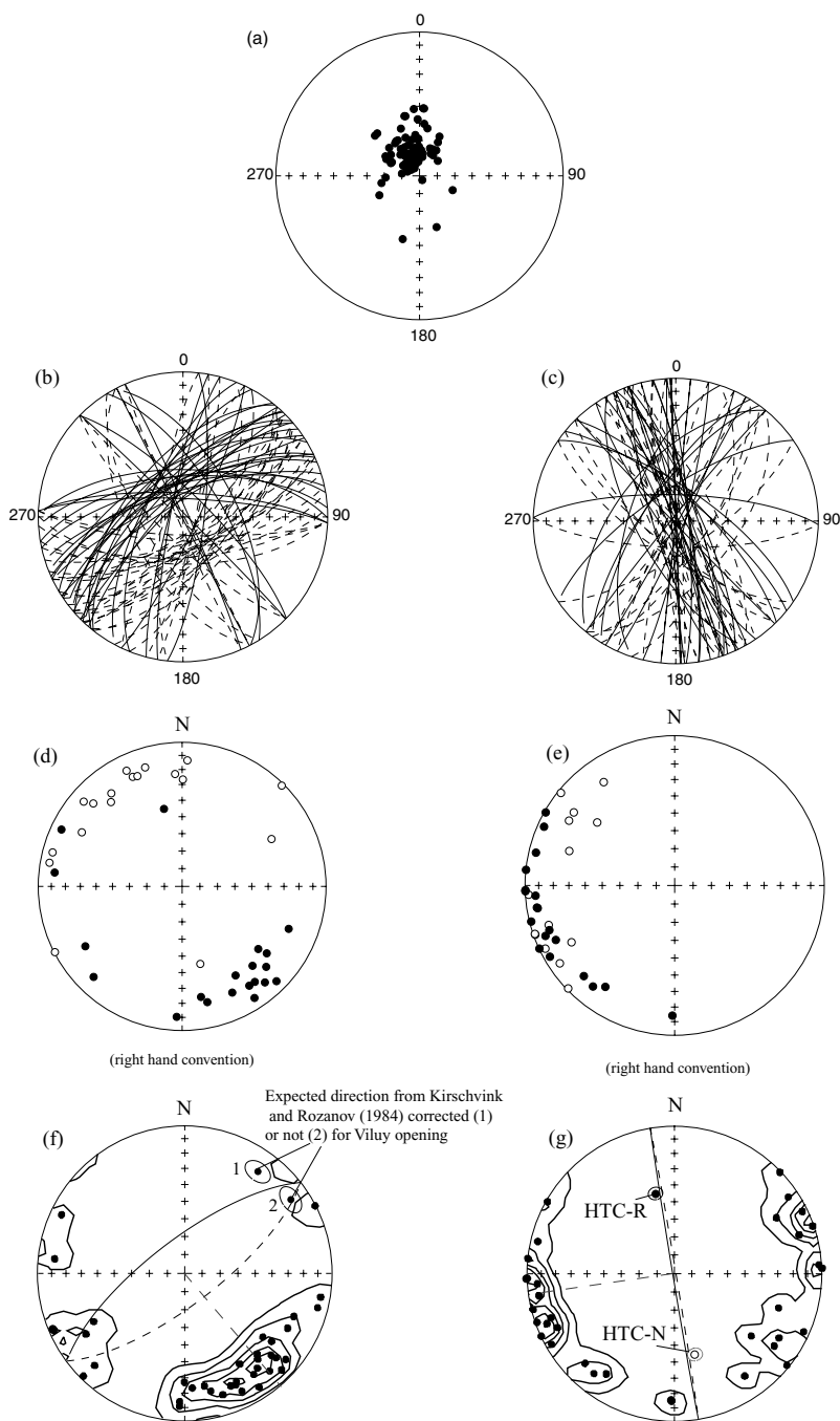
Figure 7. Equal-area projection of directions isolated in the low to middle temperature range in samples from the lower part of the Khorbusuonka section (a). (b) and (c) great circles determined from samples from the lower (b) and upper (c) parts of the section. (d) and (e) directions of the normals to the demagnetization planes isolated within the lower (d) and upper (e) parts of the section, and corresponding density diagrams (f and g, respectively). Same conventions as in Fig. 3.
