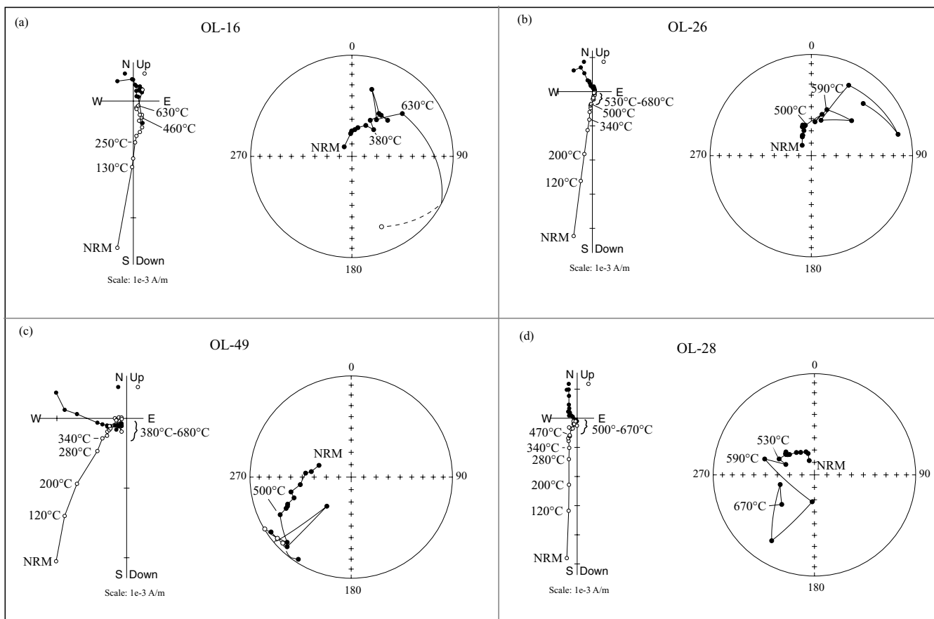
Figure 9. Demagnetization diagrams obtained from samples taken in the Erket Formation from the Olenek section. These samples exhibit the ‘ \alpha ’ (a and b) and ‘ -\alpha ’ (c and d) behaviours previously defined based on results from the Khorbusuonka section.
